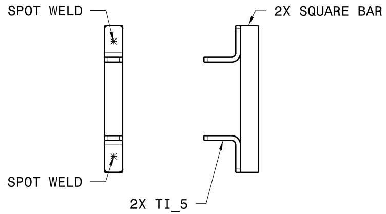
END_SUPPORT_ASSY
